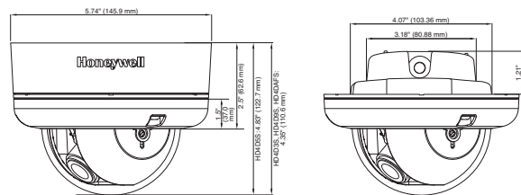
HD4D Series Dimensions
