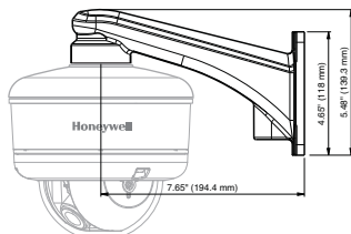
HD4CHIP-WK Wall Mount
