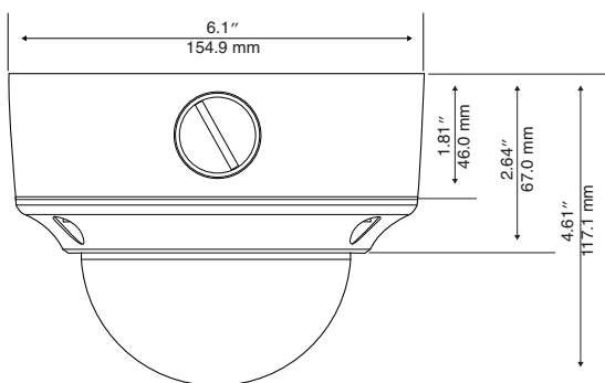
HD55IP Dimensions
